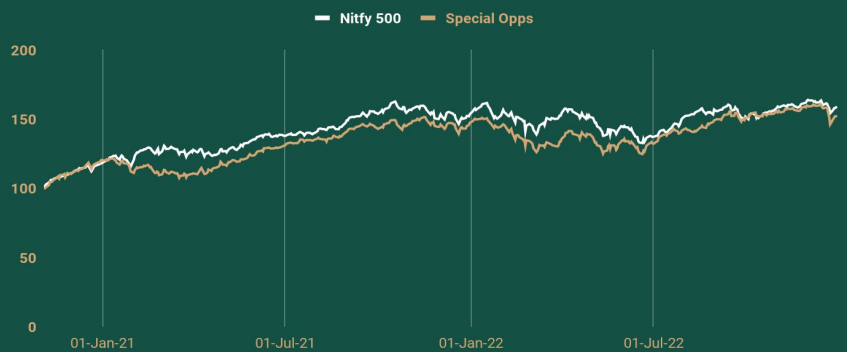
NIFTY 500 NAV and Special Opps
